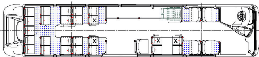
27 seats + driver + "wheelchair" space
