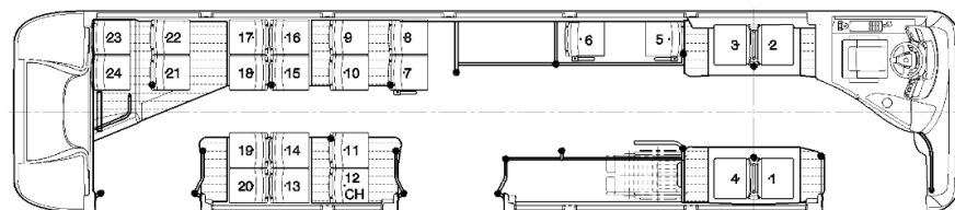
24 seats + driver + "wheelchair" space
