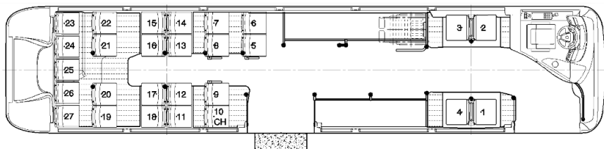
27 seats + driver + "wheelchair" space
