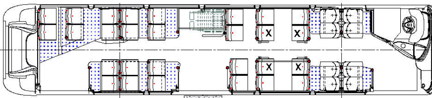
27 seats + driver + "wheelchair" space
